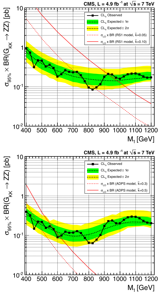
Fig. 3. Observed (black solid lines) and expected (black dashed line) 95% CL upper limits on the cross section times branching fraction for G_{KK} \rightarrow ZZ , obtained with the CL_s technique. The graviton signal was generated according to the model in [1] (RS1, top) and [10] (ADPS, bottom). The 68% and 95% ranges of expectation for the background-only model are also shown with green (darker) and yellow (lighter) bands surrounding the expected upper limit line, respectively. The predicted product of the graviton cross section and the branching fraction for different values of \tilde{k} are shown as red solid and dashed curves. (For interpretation of the references to color in this figure legend, the reader is referred to the web version of this Letter.)
