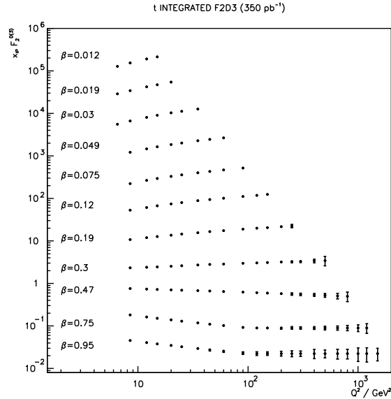
Fig. 1. Expected precision for 350 \text{ pb}^{-1} on F_2^{D(3)}(\beta, Q^2, x_P) at x_P = 0.017 , integrated over |t| < 0.8 \text{ GeV}^2 , measured in the region 0.011 < x_P < 0.024 . The data points at different \beta are scaled by arbitrary factors for visibility.
