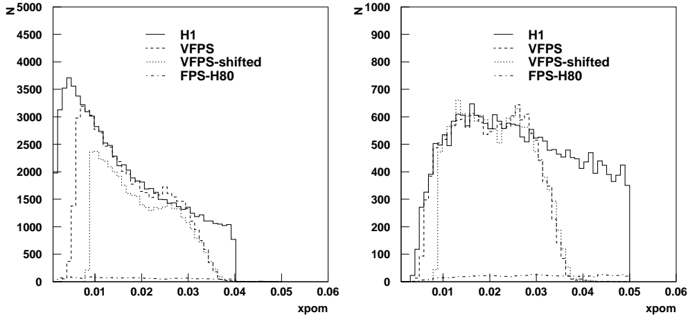
Fig. 2. x_P distribution of charm (left) and dijet (right) electroproduction events observable in H1. The full lines show the distribution for the full H1 central detector acceptance. The subset of events tagged by the VFPS is given by the dotted lines and the events tagged by the FPS are also shown. The overall normalisation is arbitrary.
