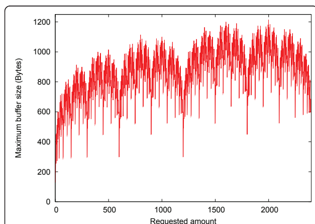
Figure 8 Measured maximal buffer occupation, 8 slots.
